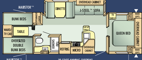
MAXISTOR™ 20-FOOT AWNING (OPTION)
